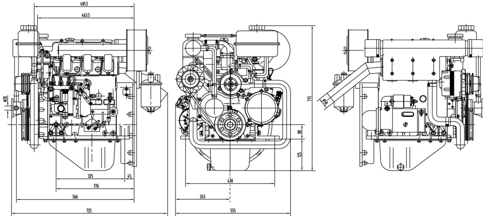
MP-327 & MP-332 Drawing
