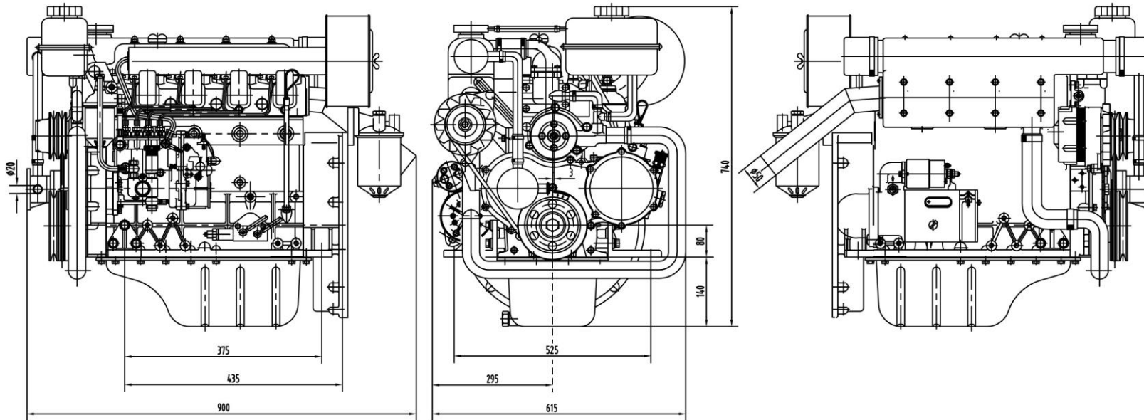
MP-458 Bobtail Drawing
