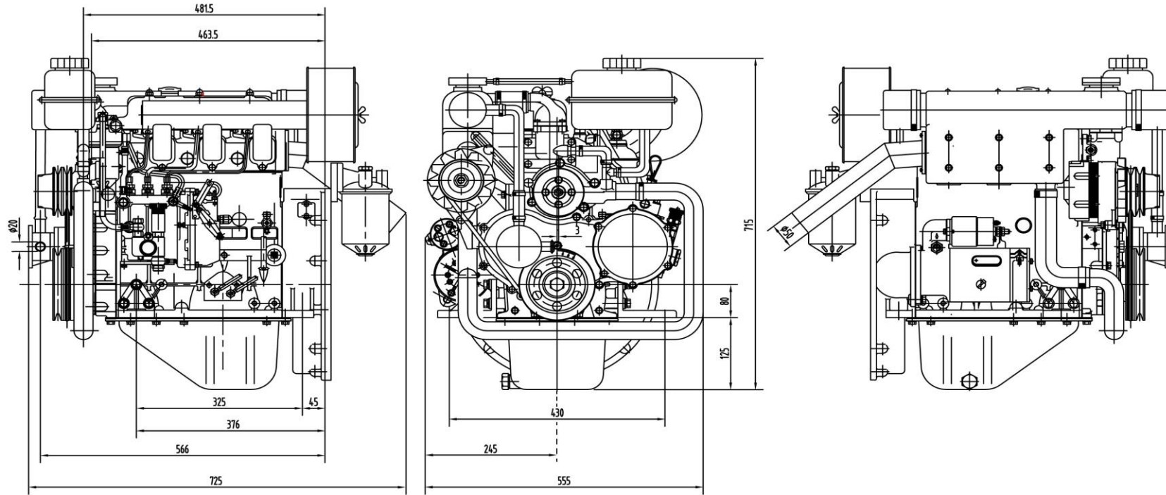
MP-327 & MP-332 Bobtail Drawing
